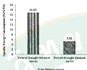
Fig. 4 specific fuel consumption
