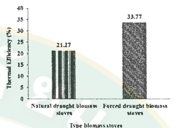
Fig. 6 thermal efficiency
