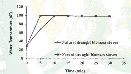
Fig. 5 hot water temperature
