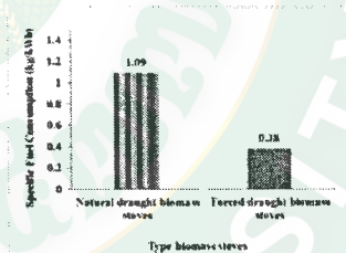
Fig.3 the specific fuel consumption
